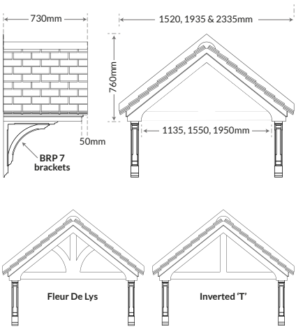
T-Bar Option: White frame with grey tiles & GRP brackets (BRP7)
