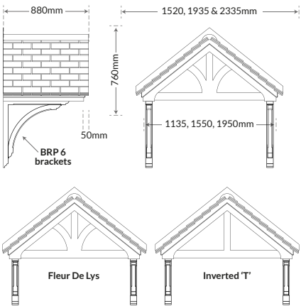
Open Option: White frame with grey tiles & GRP brackets (BRP6)
